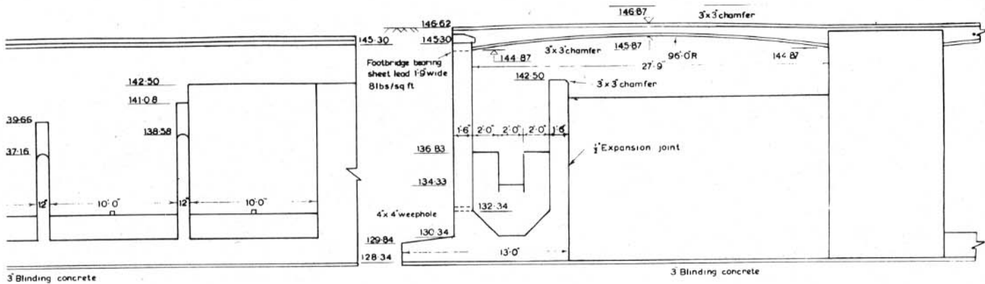
SECTION CC
