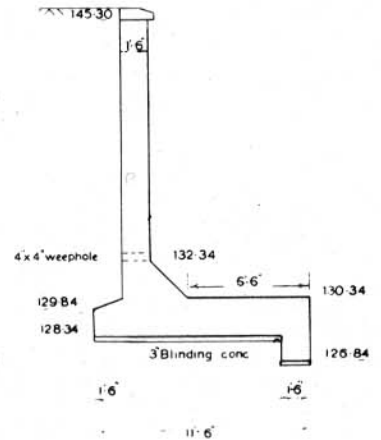
SECTION GG
