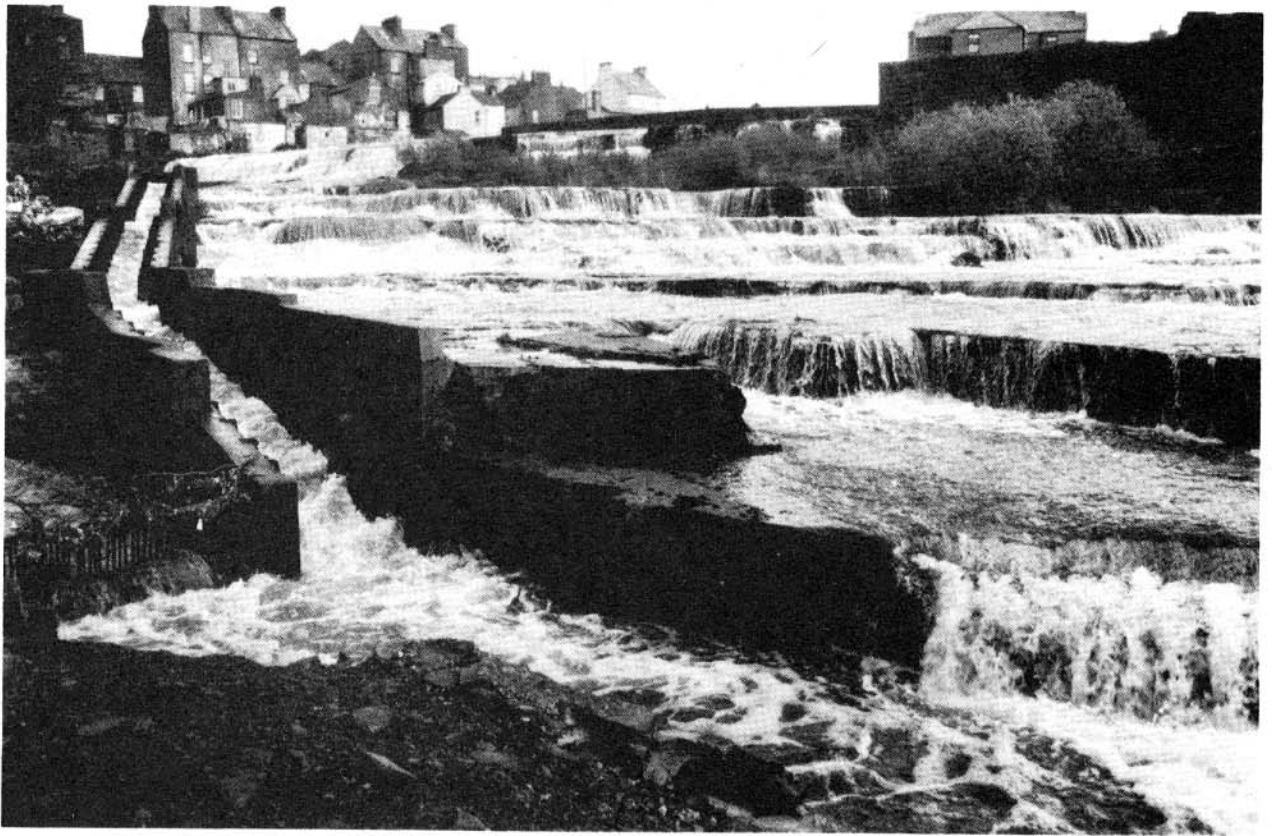
Figure 19 A view up part of the extensive Denil fish pass complex at Ennistymon on the River Inagh in the Republic of Ireland.
